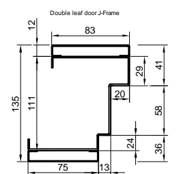
Fram fastening with screws type-J
